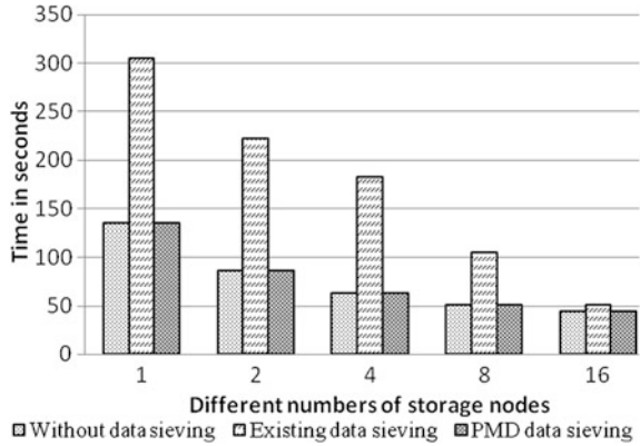
Fig. 5 Execution time for access scenario 2 (fixed client processes)
