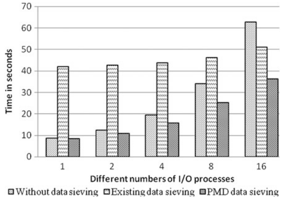
Fig. 1 Execution time for access scenario 1 (fixed storage nodes)
