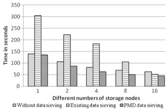
Fig. 4 Execution time for access scenario 1 (fixed client processes)
